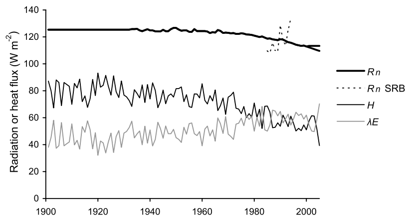
Figure 10. Time series of net radiation and heat fluxes in the Krishna Basin, 1901–2005, including the effects of the ABC and irrigation. The two different R_n lines indicate estimates for 1999–2005 based on the average of the late 1990s and extrapolation of the linear trend over 1990–1998. R_n SRB is radiation from NASA's Surface Radiation Budget. GHG forcing and interannual variability in R_n due to sources other than aerosols are not included in the calculation of R_n or H .
